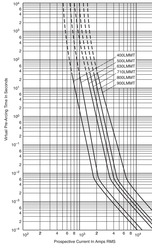
Time-current curve
