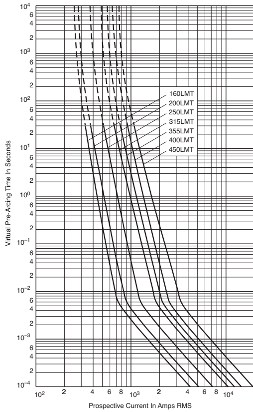
Time-current curve
