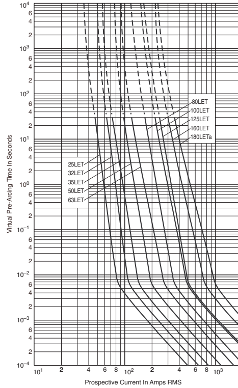
Time-current curve
