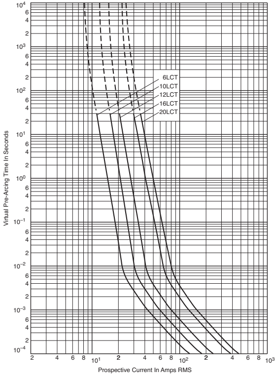
Time-current curve
